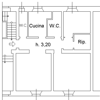
PIANO TERRENO
